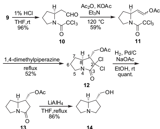
Scheme 3. Synthesis of (–)-trachelanthamidine ( 14 ) using radical cyclization of 11 .
