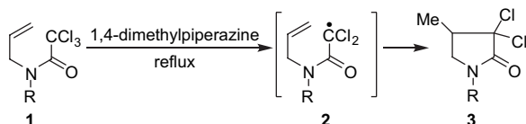
Scheme 1. Radical cyclization of 1 in 1,4-dimethylpiperazine to give 3 .
