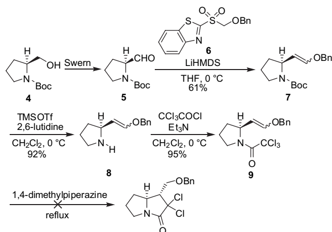
Scheme 2. Preparation and attempted radical cyclization of 9 .
